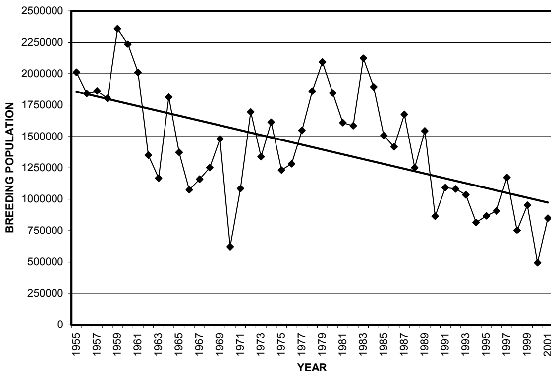
Figure 5. Trends in breeding populations of scoters (all species combined) in North America.
