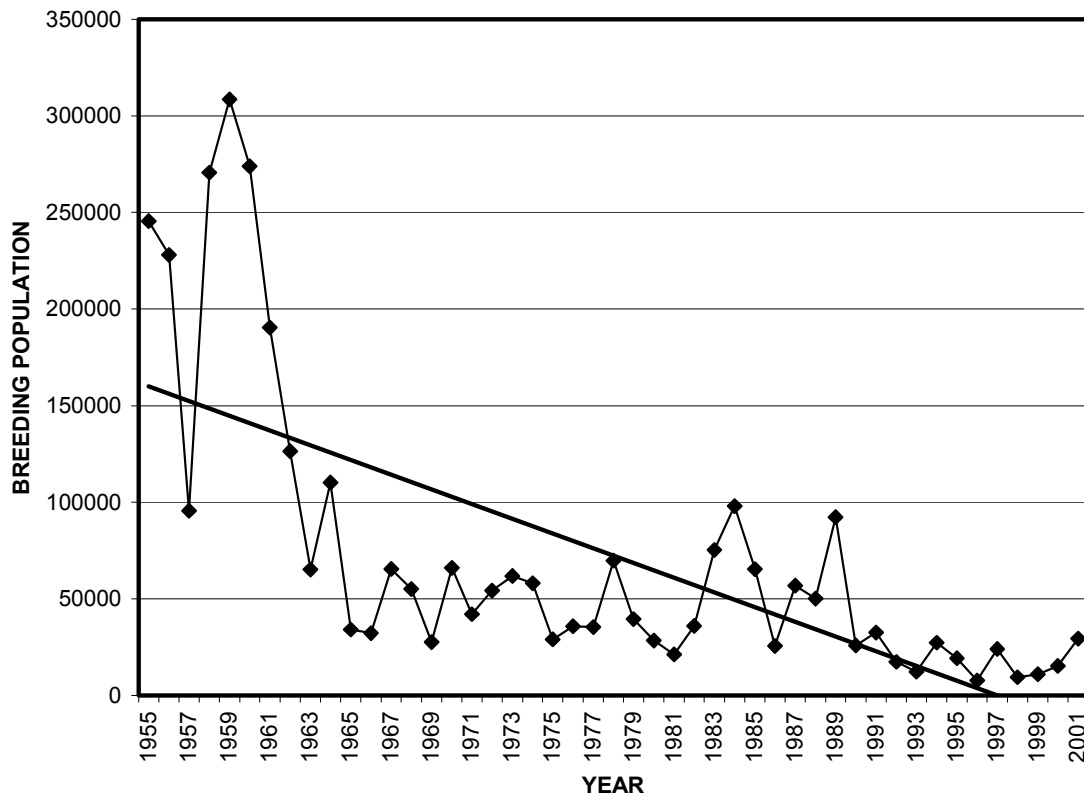
Figure 4. Trends in breeding populations of scoters (all species combined) in northern Alberta.
