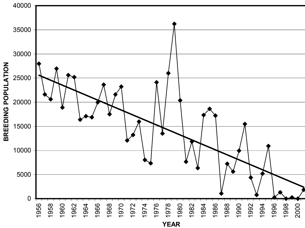
Figure 3. Trends in breeding populations of the white-winged scoter in southern Alberta.
